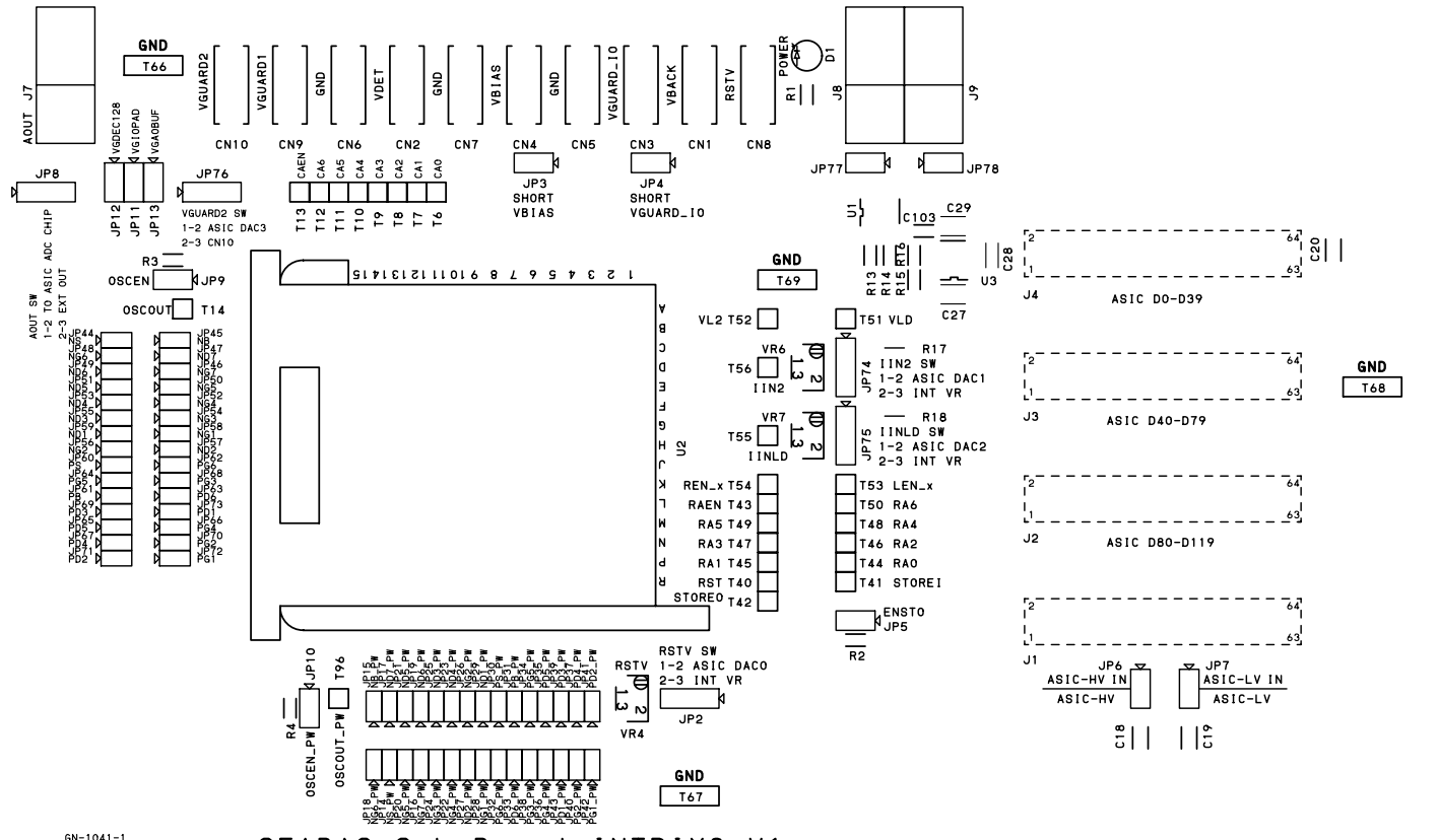
SEABAS Sub Board INTPIX3 V1
