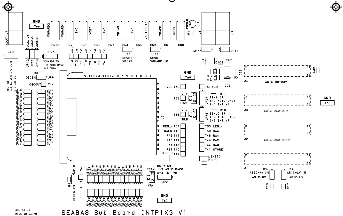
SEABAS Sub Board INTPIX3 V1
